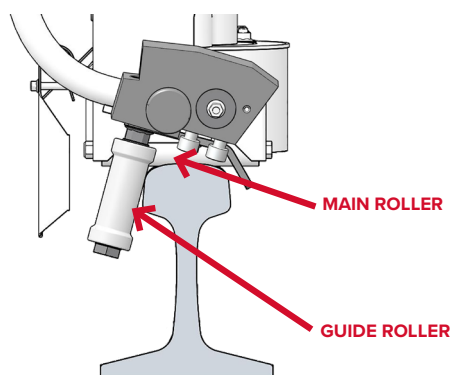
TYPICAL RAIL
